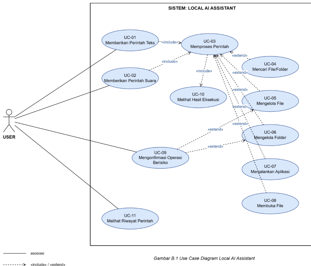
Gambar B.1 Use Case Diagram Local AI Assistant
